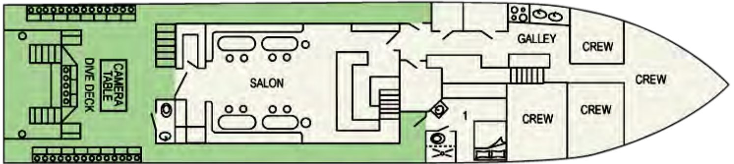
MAIN DECK
