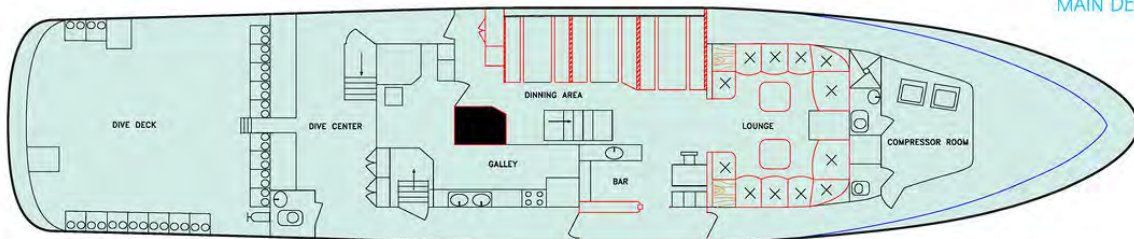
MAIN DECK
